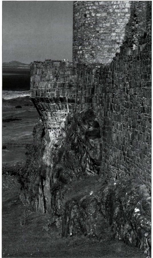
A corbelled latrine turret on the outer south wall at Harlech. This is reminiscent of Savoyard work at La Bâtiaz in Switzerland. (CADW)
