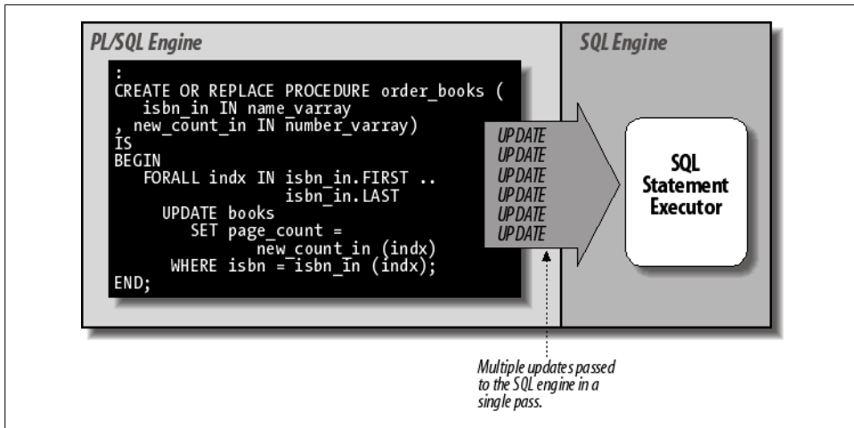
Figure 21-3. One context switch with FORALL
