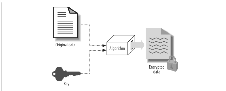
Figure 23-1. Encryption basics
