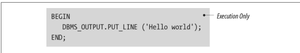
Figure 3-3. An anonymous block without declaration and exception sections
