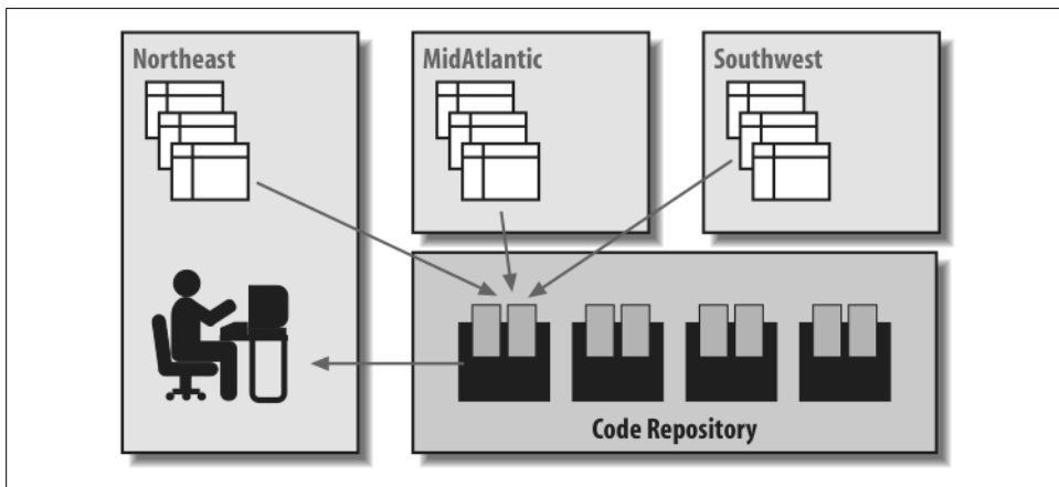
Figure 24-5. Use of invoker rights model
