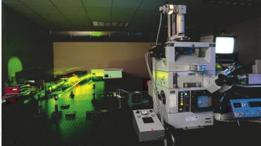
MICROBEAM SYSTEM for laser scissors incorporates a pulsed laser and a phase contrast microscope. The pulses, lasting 10 nanoseconds, are visible as the discrete light bursts along the line of the laser path. The system shown is the immediate predecessor to the confocal ablation trapping system, which has enclosed beams that are not visible.
