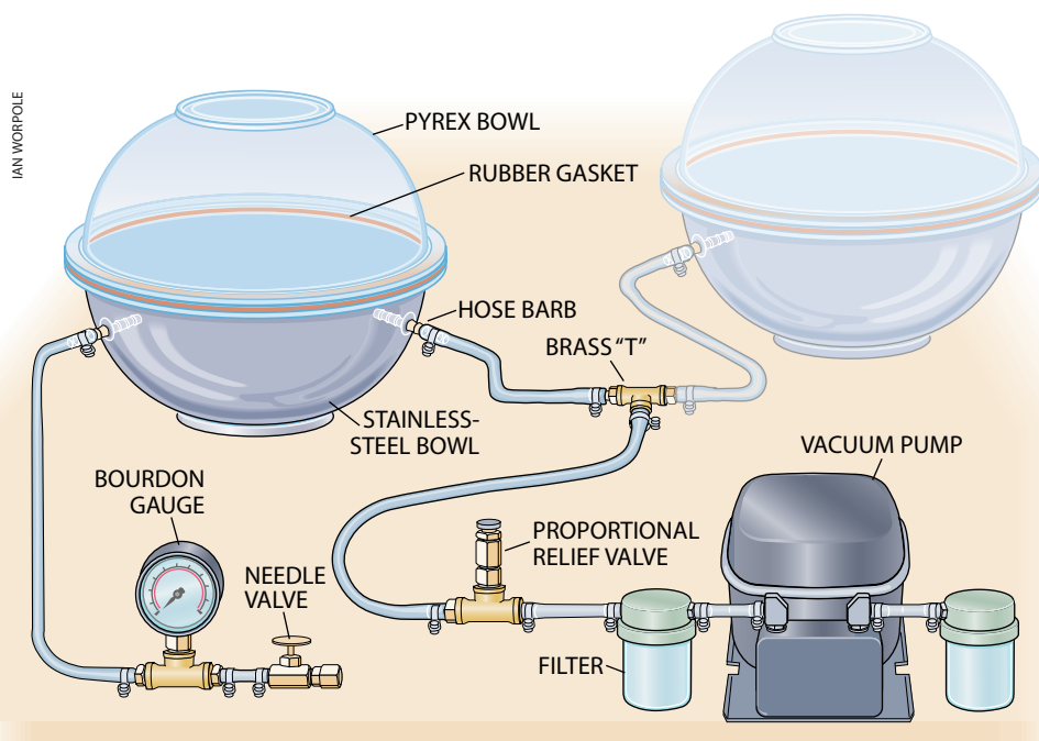
MIXING BOWLS OF GLASS AND METAL attached to a vacuum pump make a spherical altitude chamber.
