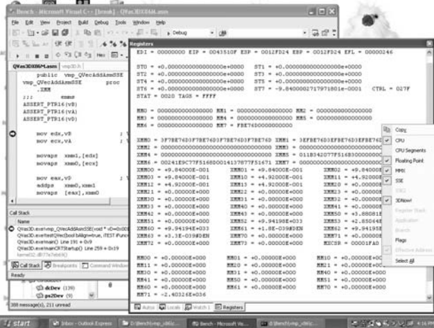
Figure 18-4: Register dump from Visual C++ .NET version 7 (3DNow! Professional Extensions). Note the 3DNow! and SSE supported registers as well as the extra pop-up menu of register type selections that you can select for your window. The enabled selections are based upon the processor type running on the computer that is being debugged.
