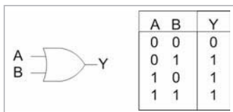
Figure 4-2: Logical OR
