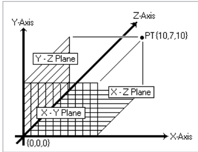
Figure 11-2: 3-dimensional Cartesian coordinate system
