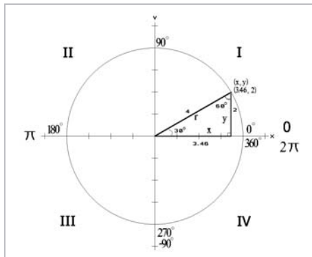
Figure 11-1: 2D geometric circle
