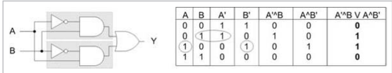
Figure 6-3: A two-gate (ANDC, OR) solution to achieve an equivalent result of a logical XOR
