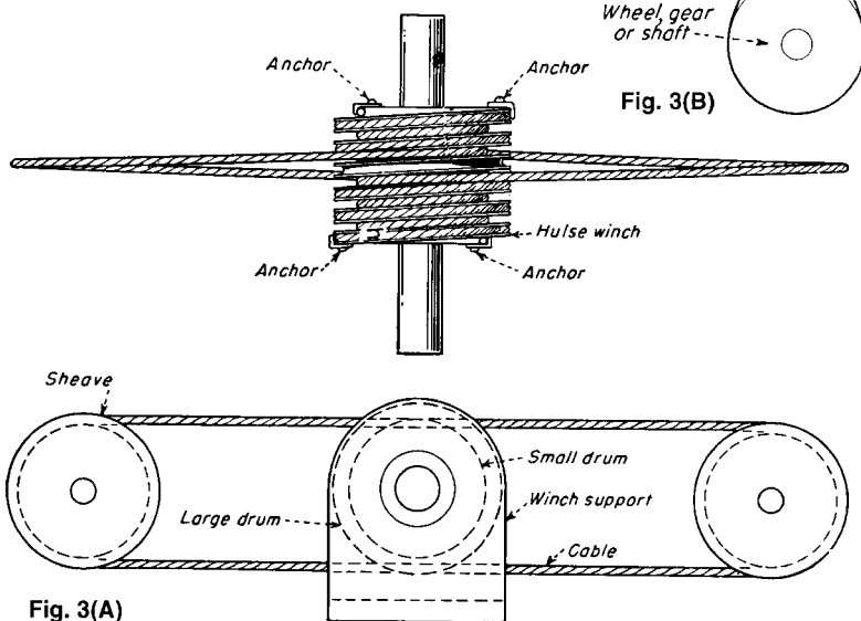
Fig. 3(A) A Hulse Winch with opposing sheaves. This arrangement, which uses two separate cables and four anchor points, can be considered as two winches back-to-back with one common set of drums. Variations in motion can be obtained by: (1) restraining in the sheaves so that when the system is rotated the drums will travel toward one of the sheaves; (2) restraining the drums and allowing the sheaves to travel. The distance between the sheaves will remain constant and is usually connected by a bar; (3) permitting the drums to move axially while restraining them transversely. When the system is rotated, drums will travel axially one pitch per revolution, and sheaves remain in the same plane perpendicular to the drum axis. This variation can be reversed by allowing sheaves to move axially; and (4) sheaves need not be opposite but can be arranged as in Fig. 3(B) to rotate a wheel.
