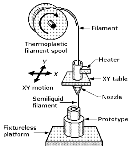
Fig. 4 Fused Deposition Modeling (FDM): A monofilament of a thermoplastic resin is unwound from a spool and passed through a heater mounted on a computer-controlled XY table. The semisolid filament is extruded from the nozzle to form the first (bottom) layer in a preset pattern by the motion of the XY table as it moves over the platform. The hot plastic binds to each successive layer as it is set down and hardened. This sequence is continued until the prototype is complete. It is then removed from the platform and sanded to improve its finish. This laserless process can form thin-walled, contoured prototypes or molds for investment casting.
