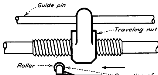
Precision type limit switch
