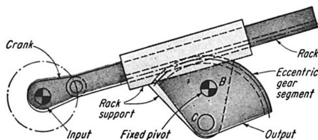
Rack and gear sector mechanism
