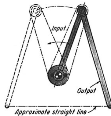
Oscillating-chain mechanism
