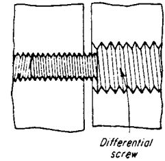
Fig. 3 A differential screw has same-hand threads but with different pitches. The relative distance between the two components can be adjusted with high precision by differential screws.
