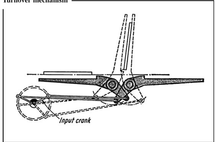
Turnover mechanism
