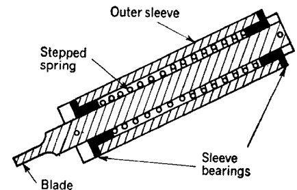
Fig. 3 Constant-torque screwdriver
