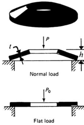
Fig. 1 Basic belleville
