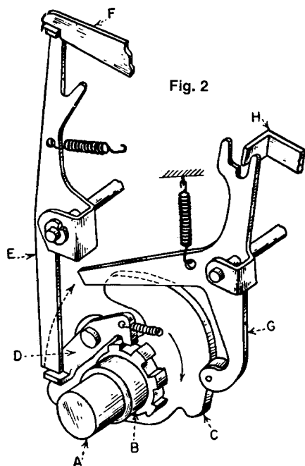
Fig. 2 A pawl and ratchet, single-cycle, dual-control clutch. The principal parts of this clutch are driving ratchet B, driven crank C, and spring-loaded ratchet pawl D. Driving ratchet B is directly connected to the motor and free to rotate on rod A. Driven crank C is directly connected to the main shaft of the machine and is also free to move on rod A. Spring-loaded ratchet pawl D is carried by crank C, which is normally held disengaged by latch E.
