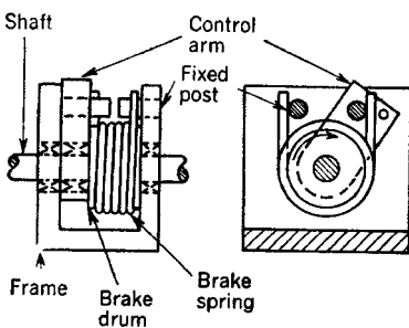
Fig. 1 Variable-torque drag brake . . .
