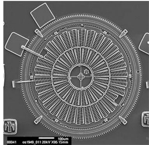
Fig. 3 Torsional ratcheting actuator. Courtesy of Sandia National Laboratories
