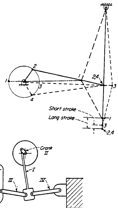
Fig. 6 A stone crusher has two toggle linkages in series to obtain a high mechanical advantage. When the vertical link I reaches the top of its stroke, it comes into toggle with the driving crank II ; at the same time, link III comes into toggle and link IV . This multiplication results in a very large crushing force.
