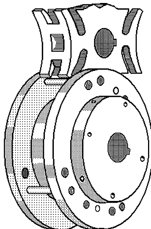
Geared star sector indexes smoothly a full 360° during a 180° rotation of the wheel, then it pauses during the other 180° to allow the wheel to catch up.
