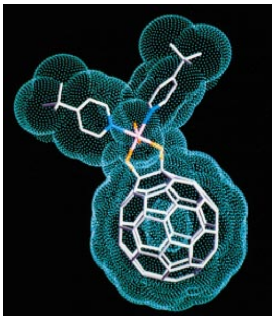
"BUNNYBALL," more formally described as C_{60}(O_4)(4\text{-tert-butylpyridine})_2 , is one of numerous chemical variations on the basic buckyball.
