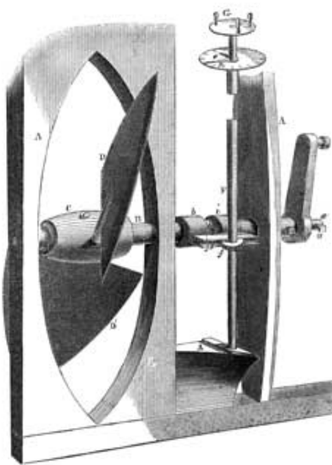
FEATHERING PROPELLER for ships, 1852
