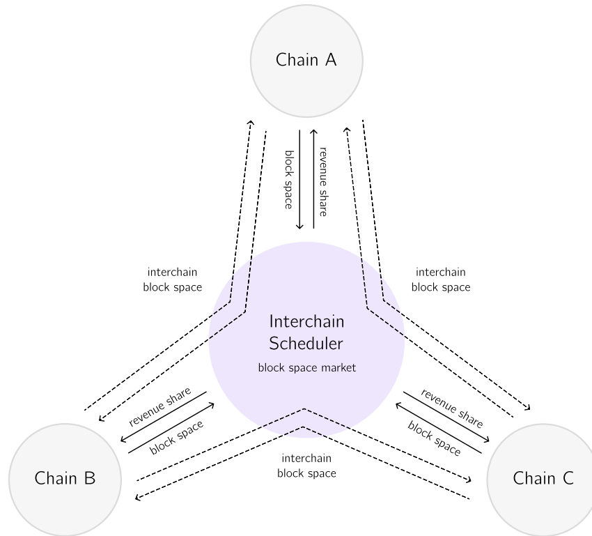
Figure 6: The Scheduler creates an in-protocol market for interchain block space, allowing chains to specify allowable MEV. Unlike other solutions that only split revenues with validators, the Scheduler also splits revenues with consumer chains.
