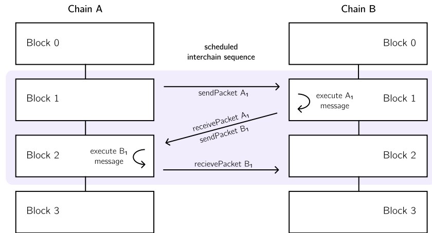
Figure 5: Depiction of a scheduled sequence of transactions occurring over multiple chains in successive blocks. The Scheduler leverages ABCI++ to enable partner chains to tokenize reservations for future block space. Those reservations are auctioned in a common MEV marketplace, enabling stronger atomicity and settlement guarantees than off-chain counterparts.
