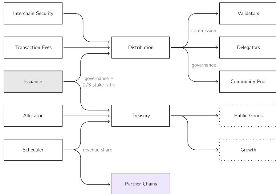
Figure 4: Interchain Security replaces issuance as a means of incentivizing validators and delegators. If the stake ratio ever drops below 2/3 , issuance will revert to the original issuance model until the ratio returns to 2/3 or higher. Issuance not directed to the distribution module is directed to the Cosmos Hub Treasury, a new capital pool managed by domain-specific councils to fund public goods and grow a resilient interchain.
