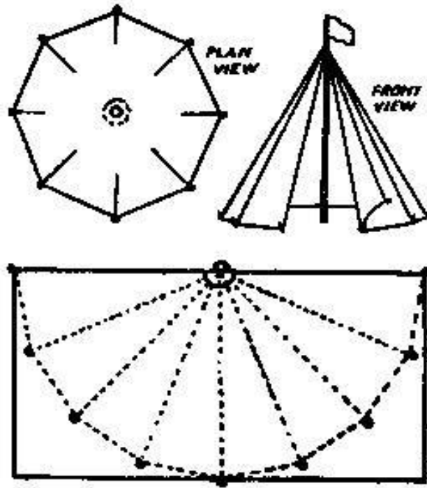
Fig. 7. Conical tent, or wigwam
