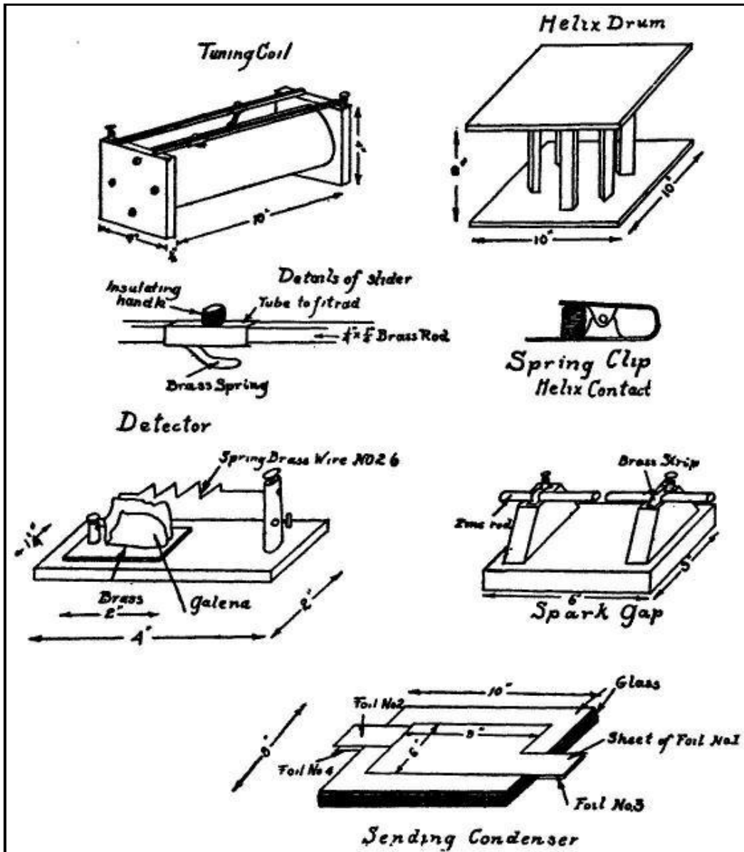
Details of instruments for field use.
