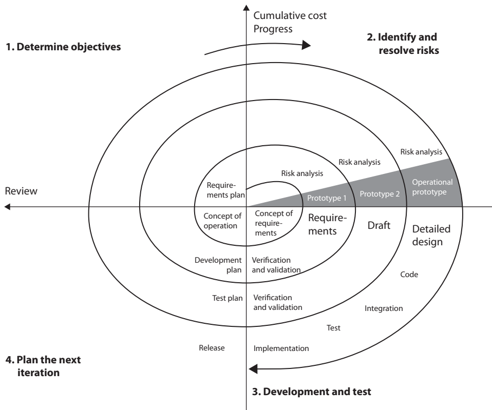
Figure 8-10 Spiral model for software development
