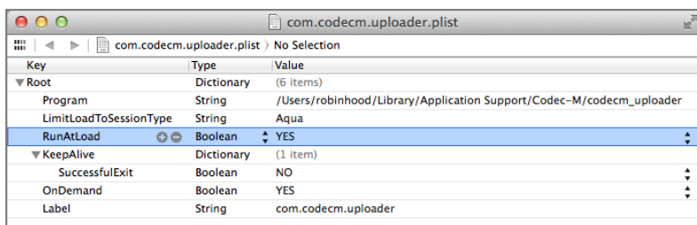
Figure 30-3: The malicious codec uses a launch agent to run at load time.
