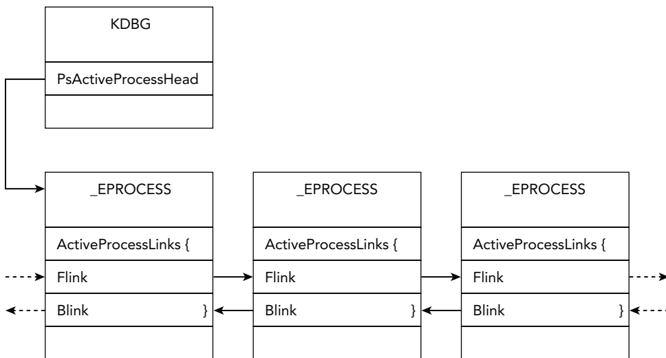
Figure 6-2: Processes are chained together in a doubly linked list pointed to by PsActiveProcessHead .
