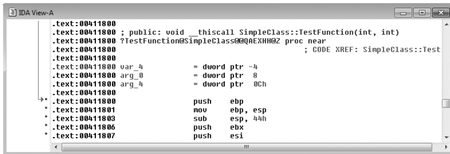
Figure 20-1: IDA Pro listing of a demangled function name
