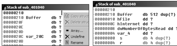
Figure 6-2L: Creating an array and fixing the stack
