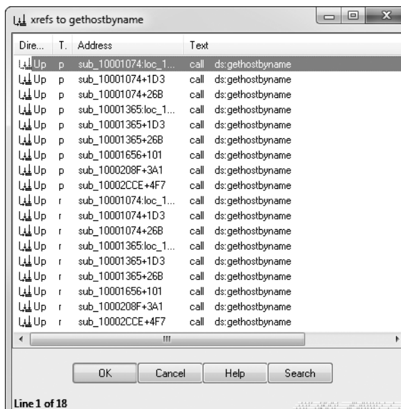
Figure 5-1L: Cross-references to gethostbyname
