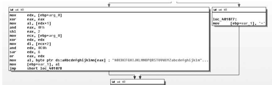
Figure 13-3L: Base64 padding
