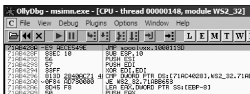
Figure 11-5L: Examining the inline hook for the send function in msimn.exe
