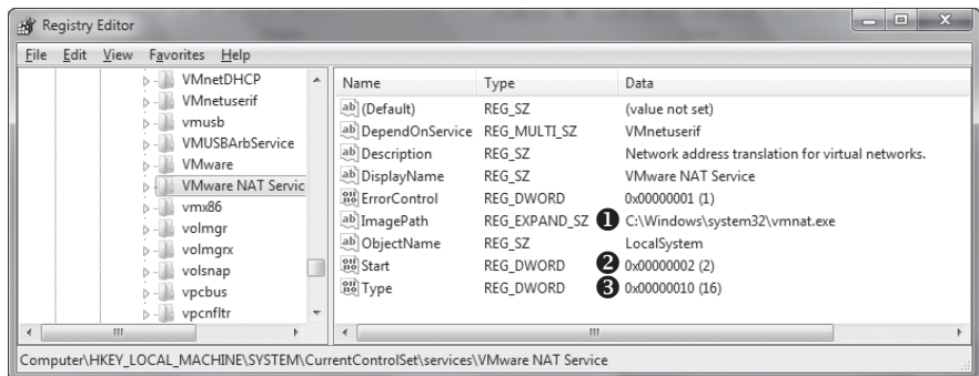
Figure 7-2: Registry entry for VMware NAT service
