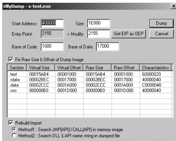
Figure 9-16: OllyDump plug-in window
