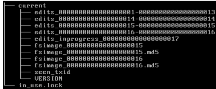
Figure 8: The NameNode tree structure
