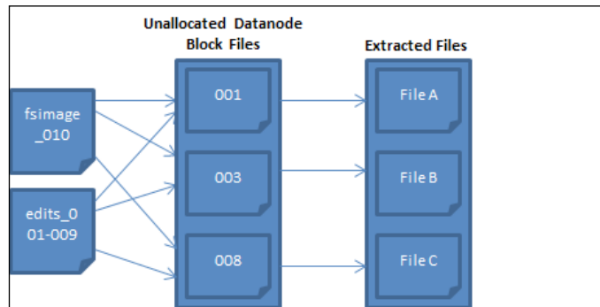
Figure 15: Unallocated DataNode block files
