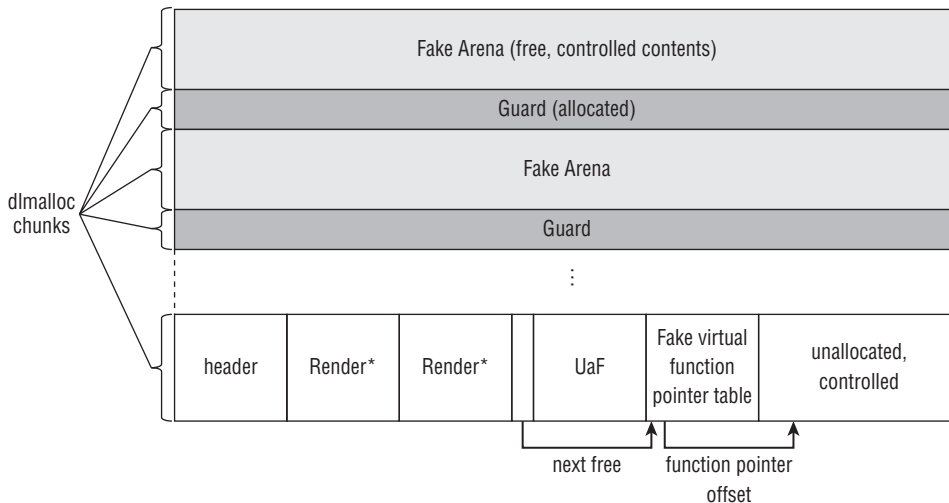
Figure 8-12: RenderArena and dmalloc state after massaging
