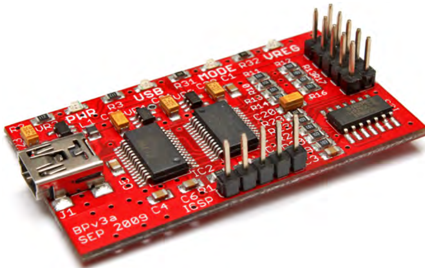
Figure 13-34: Bus Pirate v3
