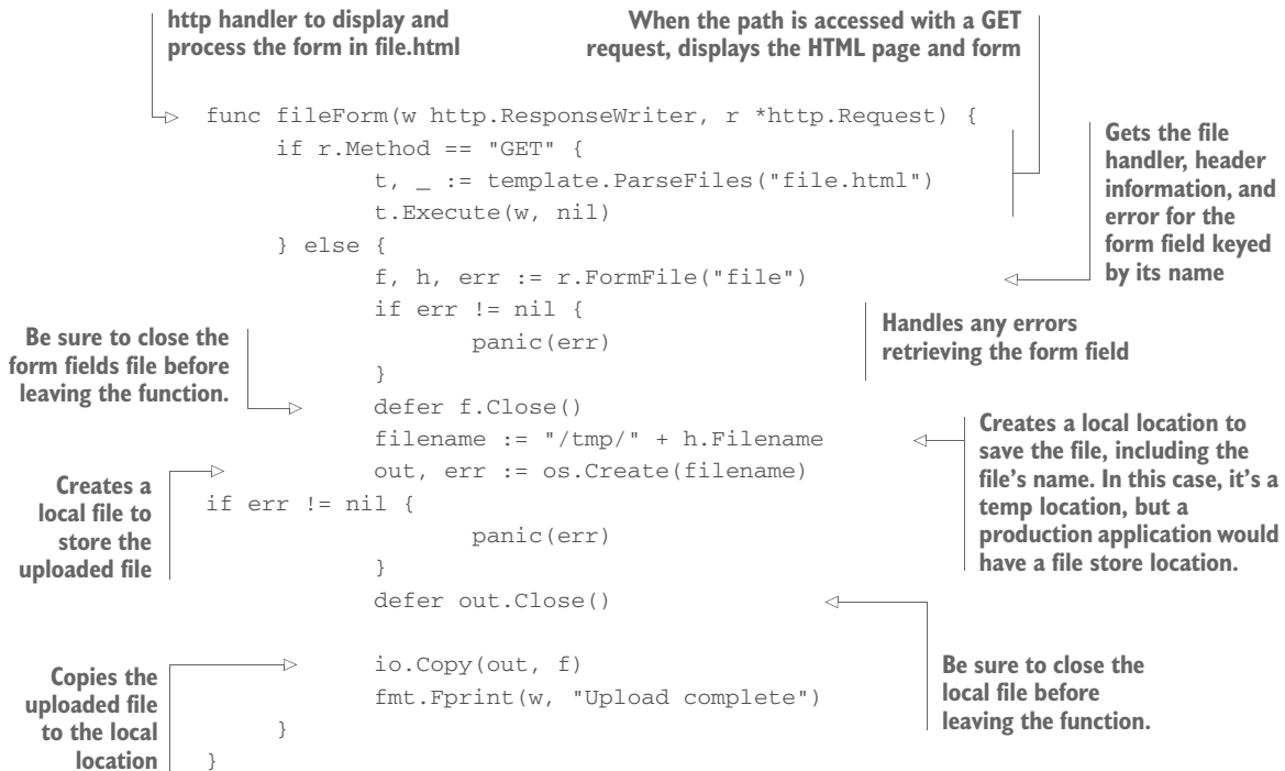
Listing 7.13 Handle a single file upload
