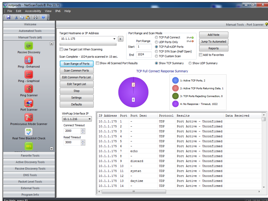
Figure 13-1: Port scanning a Linux host with NetScan- Tools Pro.
