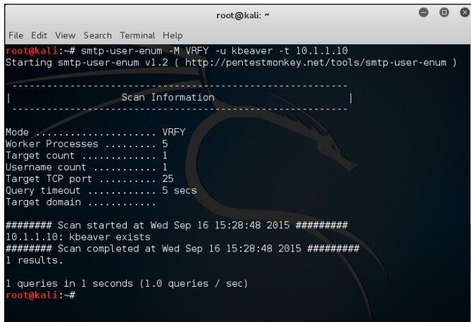
Figure 14-8: Using smtp-user-enum for gleaning e-mail addresses.
