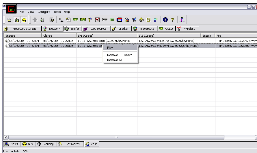
Figure 13-16: Using Cain & Abel to capture, record, and playback VoIP con- versations.
