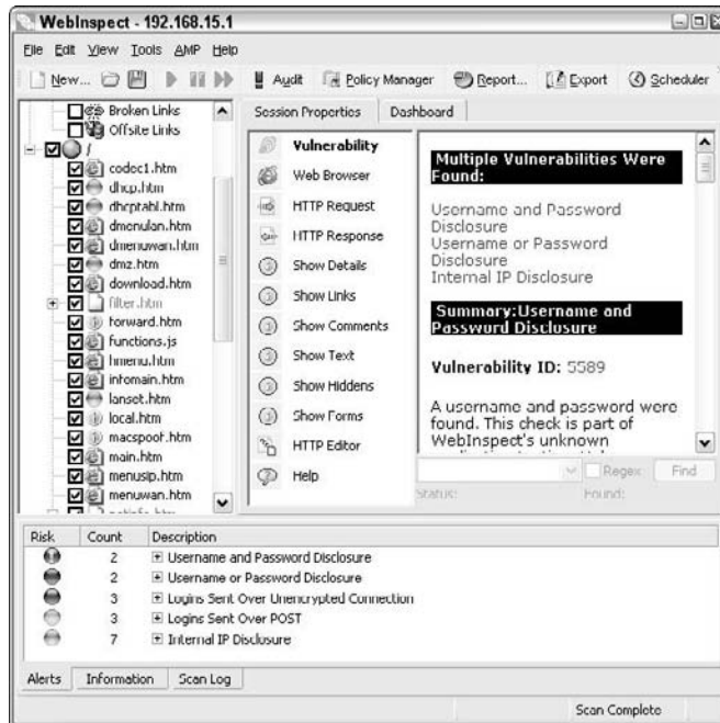
Figure 13-14: Websinspect scan of a VoIP network adapter showing several weaknesses.
