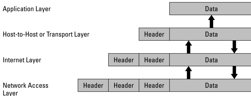
Figure 11-1: TCP/IP Encapsulation.
