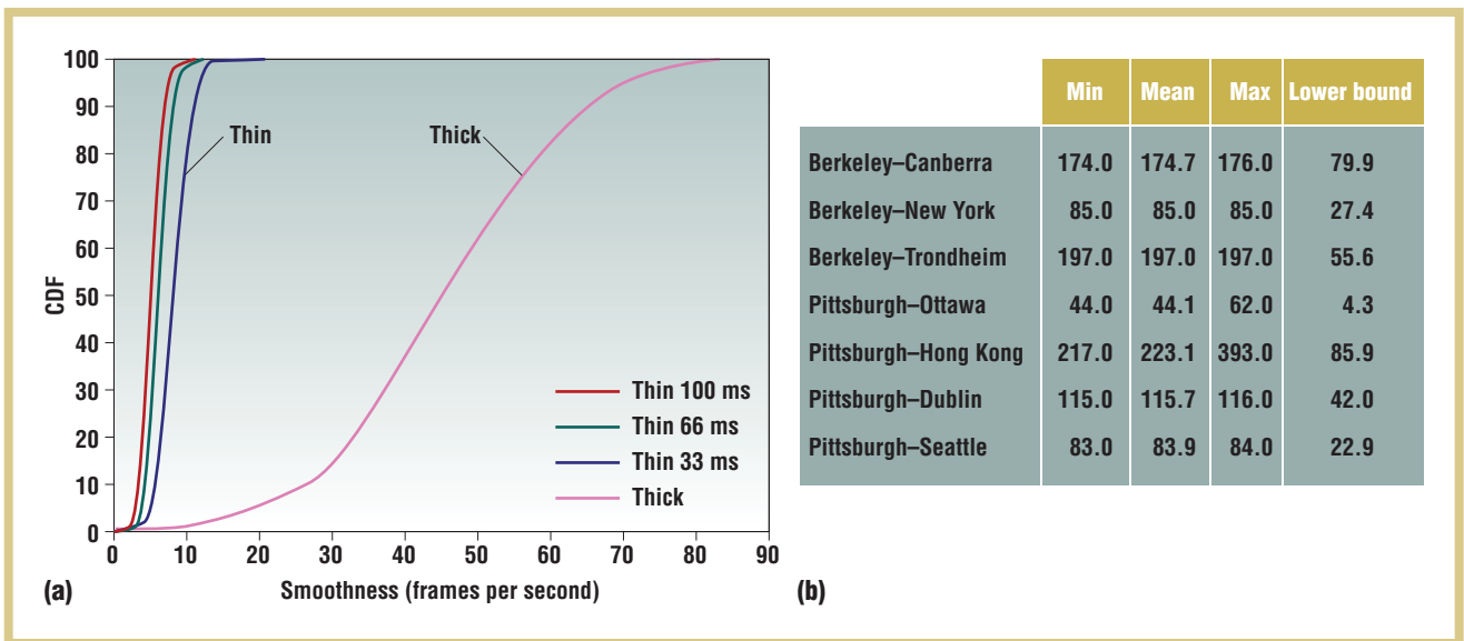
Figure 2. Network latency hurts interactive performance even with good bandwidth. (a) A highly interactive visualization application’s measured output frame rate under two different configurations: thick (a local machine with hardware graphics acceleration) and thin (a remote compute server on a 100 Mb/s network, with round-trip times ranging from 33 ms to 100 ms). (b) Measured Internet2 round-trip times between representative sites confirm that the 33–100 ms range lies well within the range of observed latencies in the real world.
